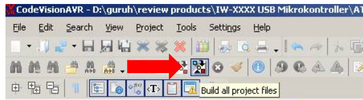
Gambar 10. Buildallprojectfiles.
