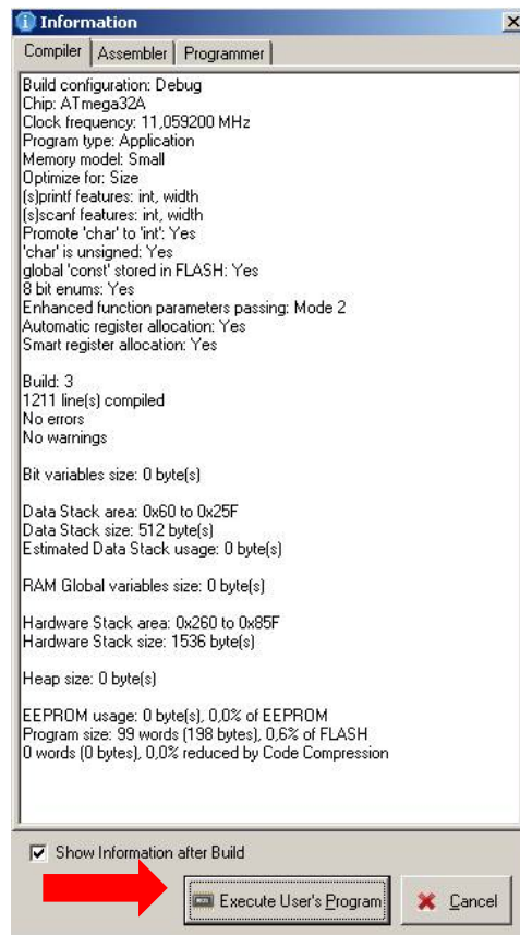
Gambar 11. ExecuteUser's Program.
