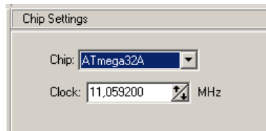
Gambar 5. ChipSettings.
