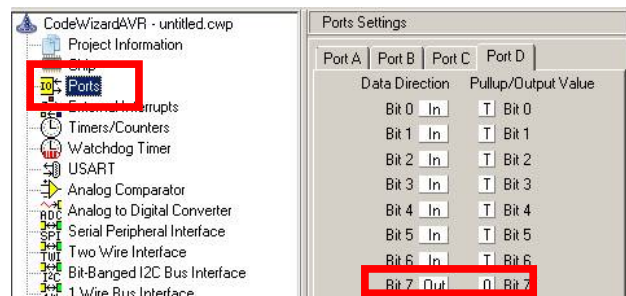
Gambar 6. Port Settings.
